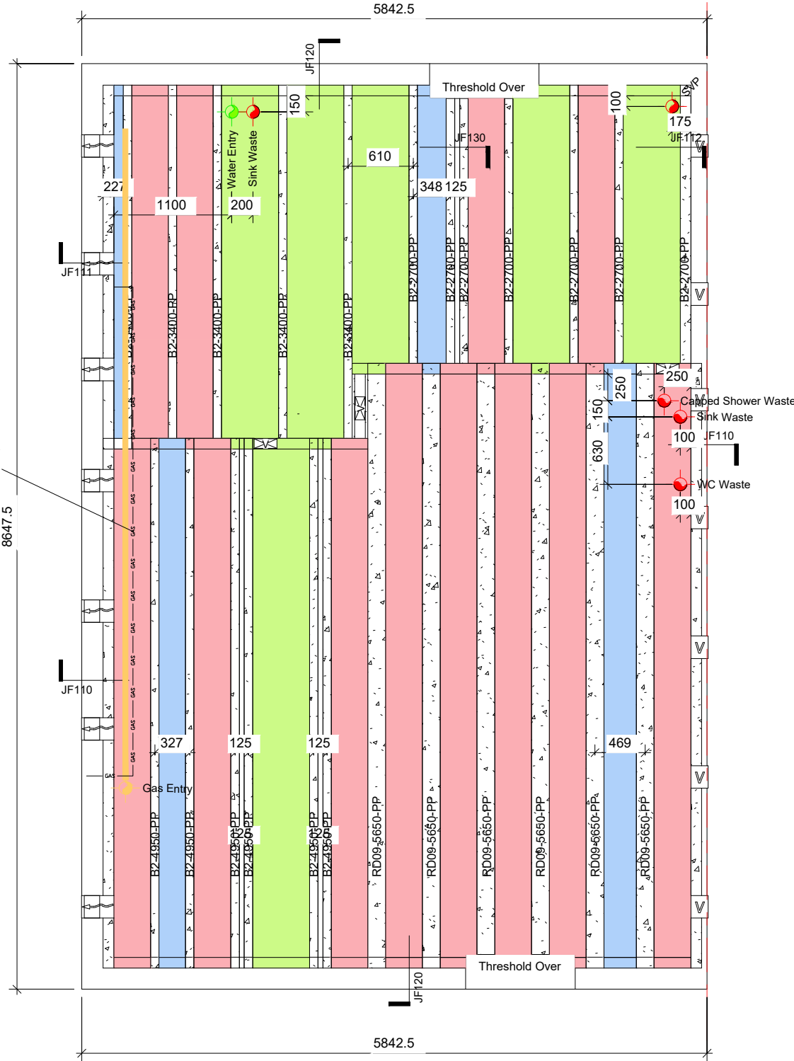
1 Beam Layout 1-50 1 : 50
